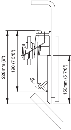
Standard TuffClamp Skirt System
